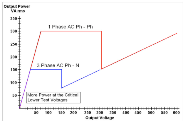
Figure 14: Voltage output power curve
