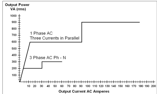
Figure 13: Current output power curve
