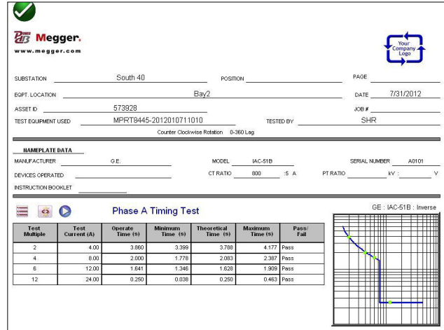
Figure 5: Test report Alstom IEC inverse timing test
