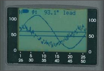
Oscillogram U and I Phase angle \varphi
